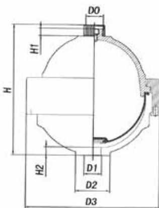
Type A Diaphragm Accumulator
